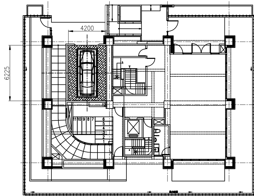
ENTRANCE FLOOR PLAN [1F]
