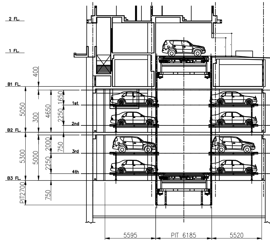
SIDE ELEVATION [ SECT. "B"- "B" ]
