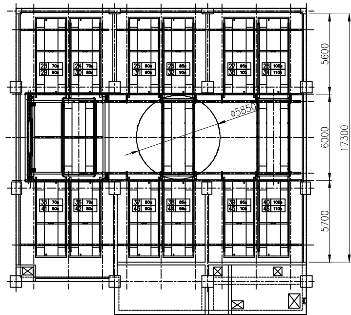
PARKING FLOOR PLAN 3 [B3]
