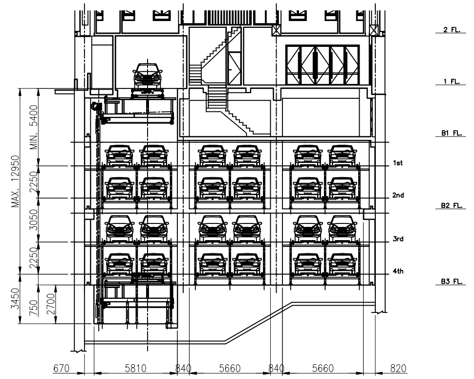
FRONT ELEVATION [ SECT. "A"- "A" ]
