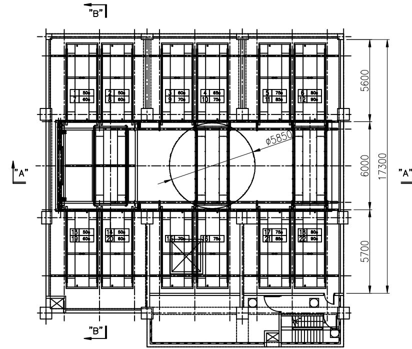
PARKING FLOOR PLAN 2 [B2]
